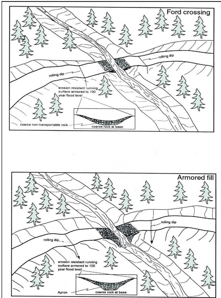
Figure X-15. CDFW California Salmonid Stream Habitat Restoration Manual.
